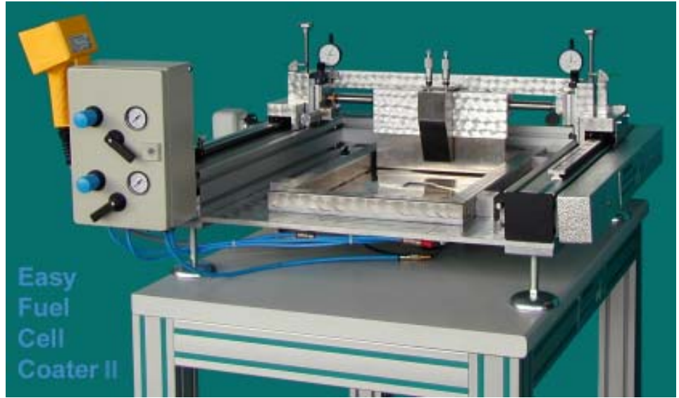
EasyCoater: Converts From Knife-Over-Air Or Knife-Over-Roller
